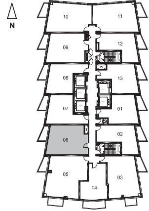
Floors 8-19
