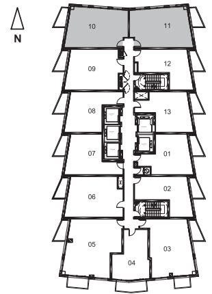
Floors 8-23, 25-PH
